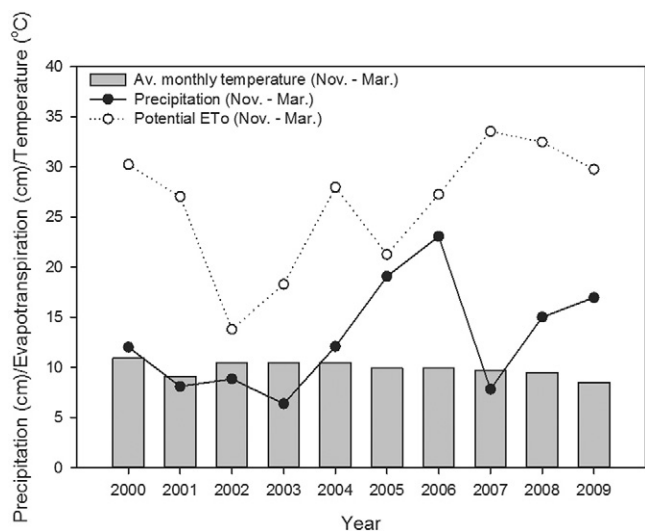
Fig. 1. Average monthly precipitation (cm), potential evapotranspiration (ET p , cm), and average monthly temperatures (°C) for Five Points, CA, study site.
