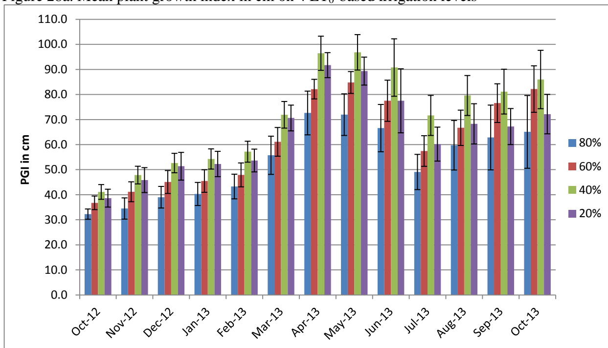
Figure 28a. Mean plant growth index in cm on 4 ET 0 -based irrigation levels
