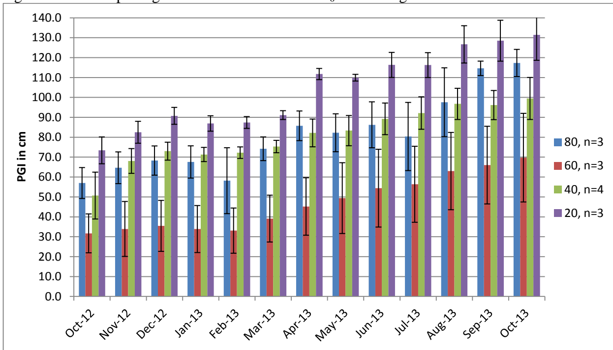
Figure 25a. Mean plant growth index in cm on 4 ET 0 -based irrigation levels
