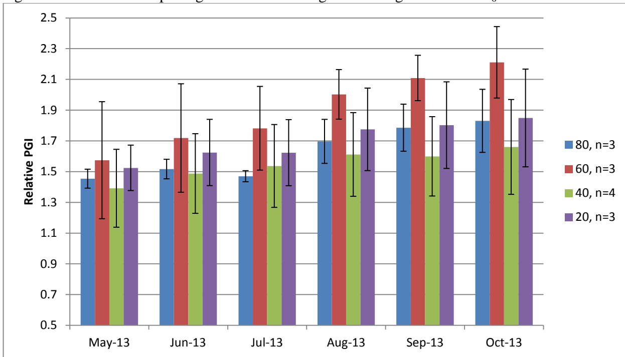
Fig. 25b . Mean relative plant growth index during deficit irrigation on 4 ET 0 -based levels
