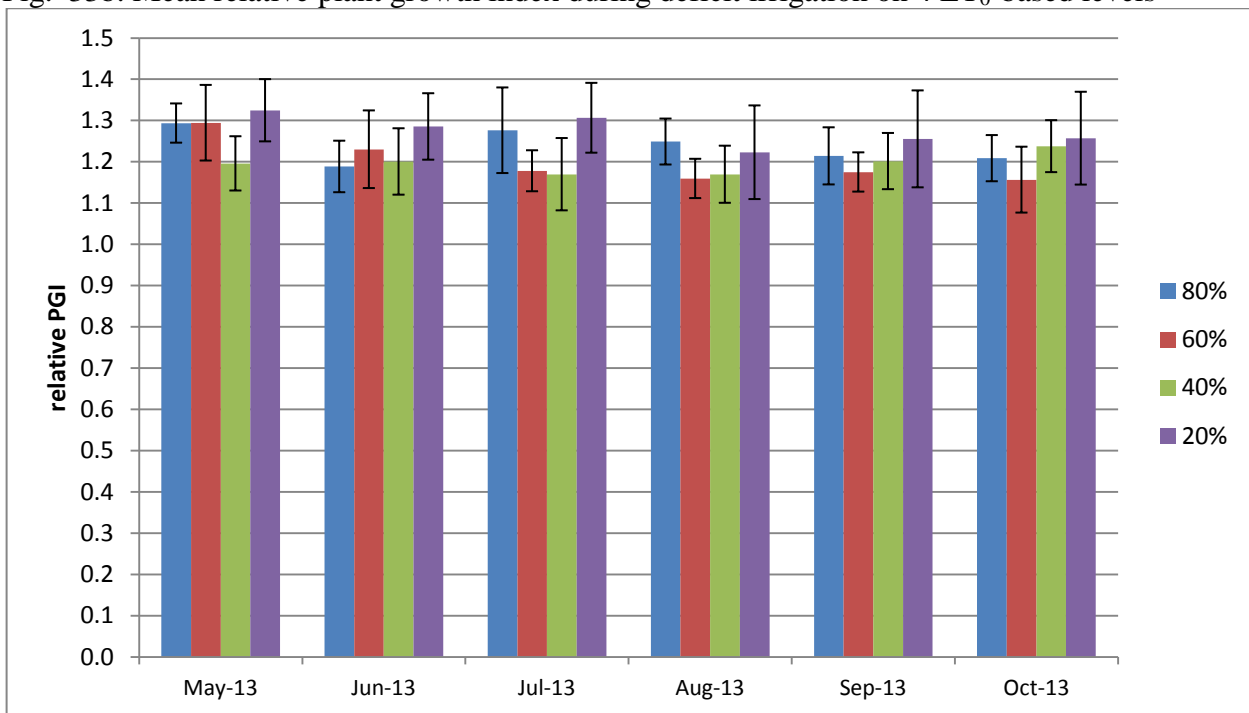
Fig. 33b. Mean relative plant growth index during deficit irrigation on 4 ET 0 -based levels
