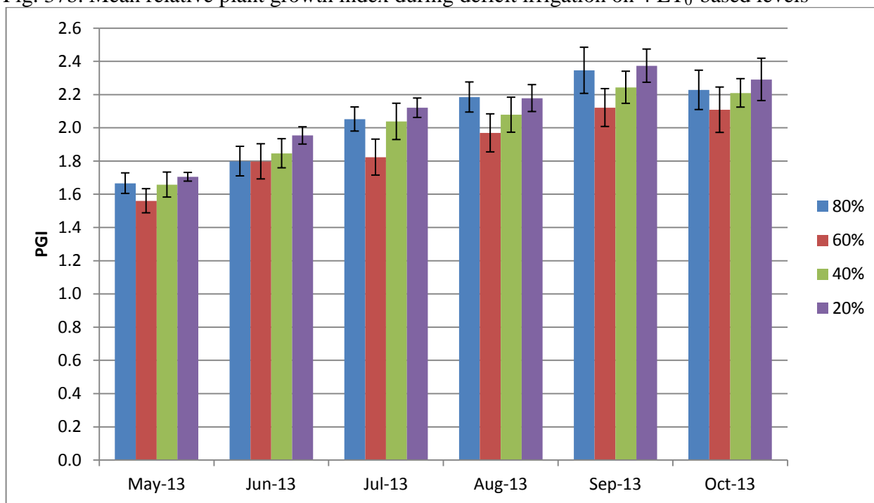
Fig. 37b. Mean relative plant growth index during deficit irrigation on 4 ET 0 -based levels
