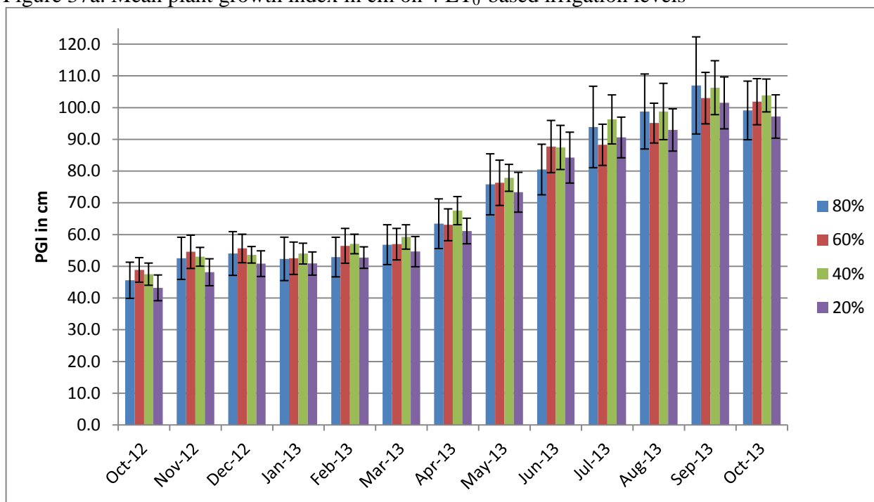
Figure 37a. Mean plant growth index in cm on 4 ET 0 -based irrigation levels
