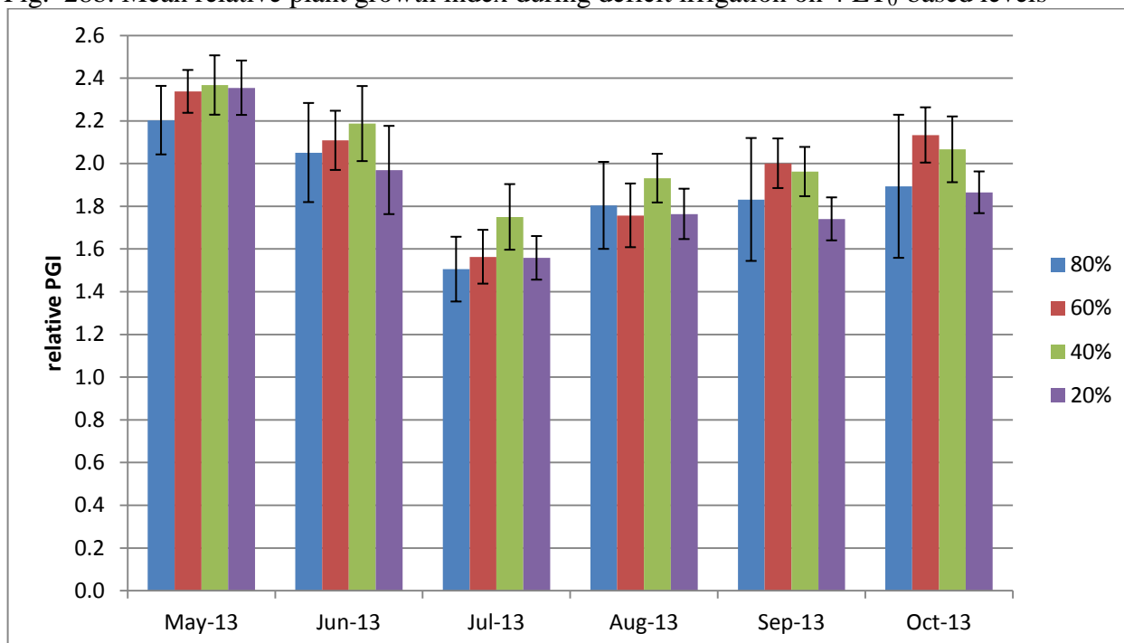
Fig. 28b. Mean relative plant growth index during deficit irrigation on 4 ET 0 -based levels
