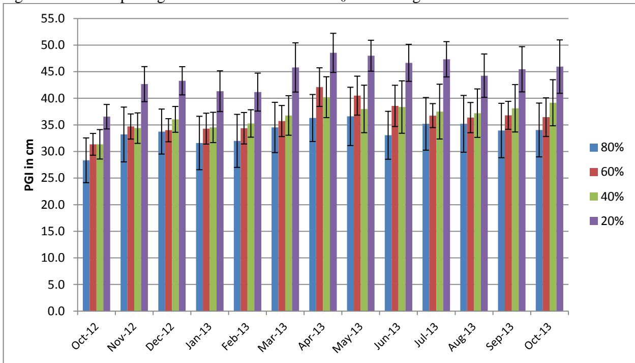
Figure 33a. Mean plant growth index in cm on 4 ET 0 -based irrigation levels
