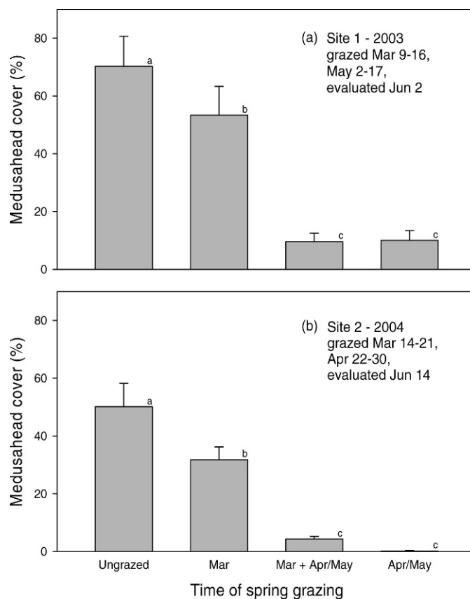
Figure 1. Medusahead at peak cover in June following first year grazing treatments for (a) site 1 (2003) and (b) site 2 (2004). Bars represent mean values + SE. Values followed by the same letter are not different (Student–Newman–Keuls test, \alpha = 0.05 ).
